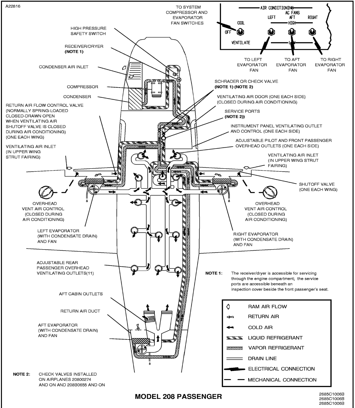
Figure 1 : Sheet 2 : R134a Air Conditioning System Schematic
