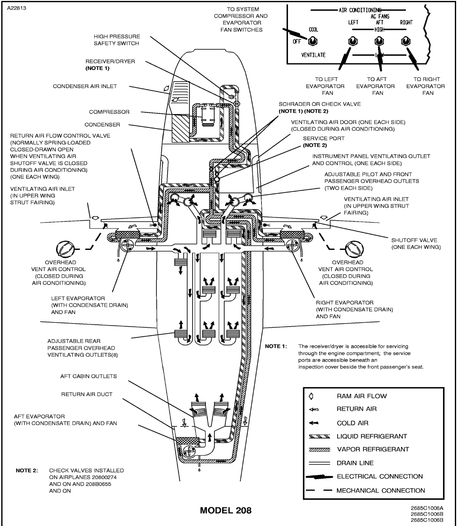
Figure 1 : Sheet 1 : R134a Air Conditioning System Schematic
